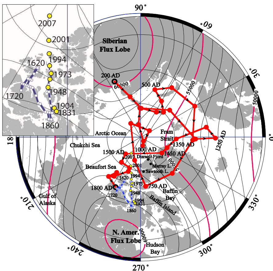
Figure 1. The reconstructed location and movement of the NMP from 200 to 1800 AD (red). The reconstruction is based on the transformation of the paleomagnetic data from Lower Murray Lake (Cook et al., 2008; Besonen et al., 2008). The historical motion of the NMP calculated from Jackson et al. (2000) is shown in blue and direct observations of the NMP as yellow points. Also observed in the figure are the North American and Siberian flux lobes. Modified from St-Onge & Stoner (2011).
